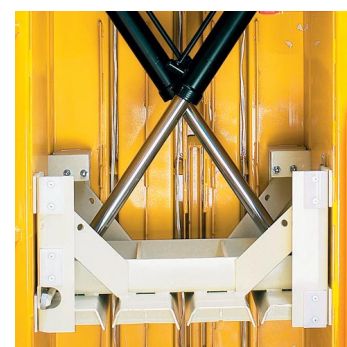
The cross cylinders ensure stable compression and a low overall height.
