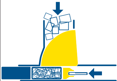
Main ram compresses material with maximum pressure. Conveyor continues to feed material to hopper.
