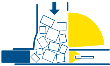
Prepress and main press in their starting positions. Press chamber full.
