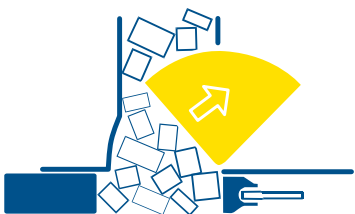
Prepress opens and material stacked on top of the prepress falls into and fills press chamber.
